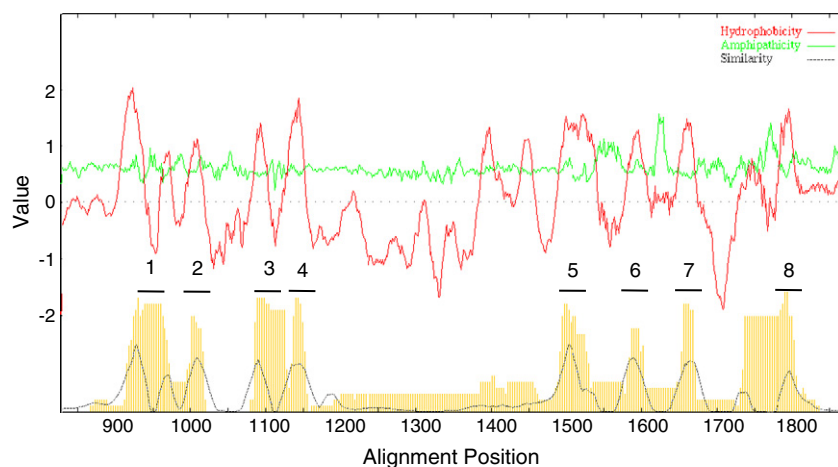
Fig. 3. Portion of average hydrophobicity, amphipathicity, and similarity (AveHAS) plots for the 189 TSUP family proteins included in this study. A magnification of the TMS-containing region is presented due to the large size of the plot which reveals 8 clear TMSs. However, as many as 12 poorly conserved peaks of hydrophobicity can be seen, suggesting that some homologues have additional TMSs.
