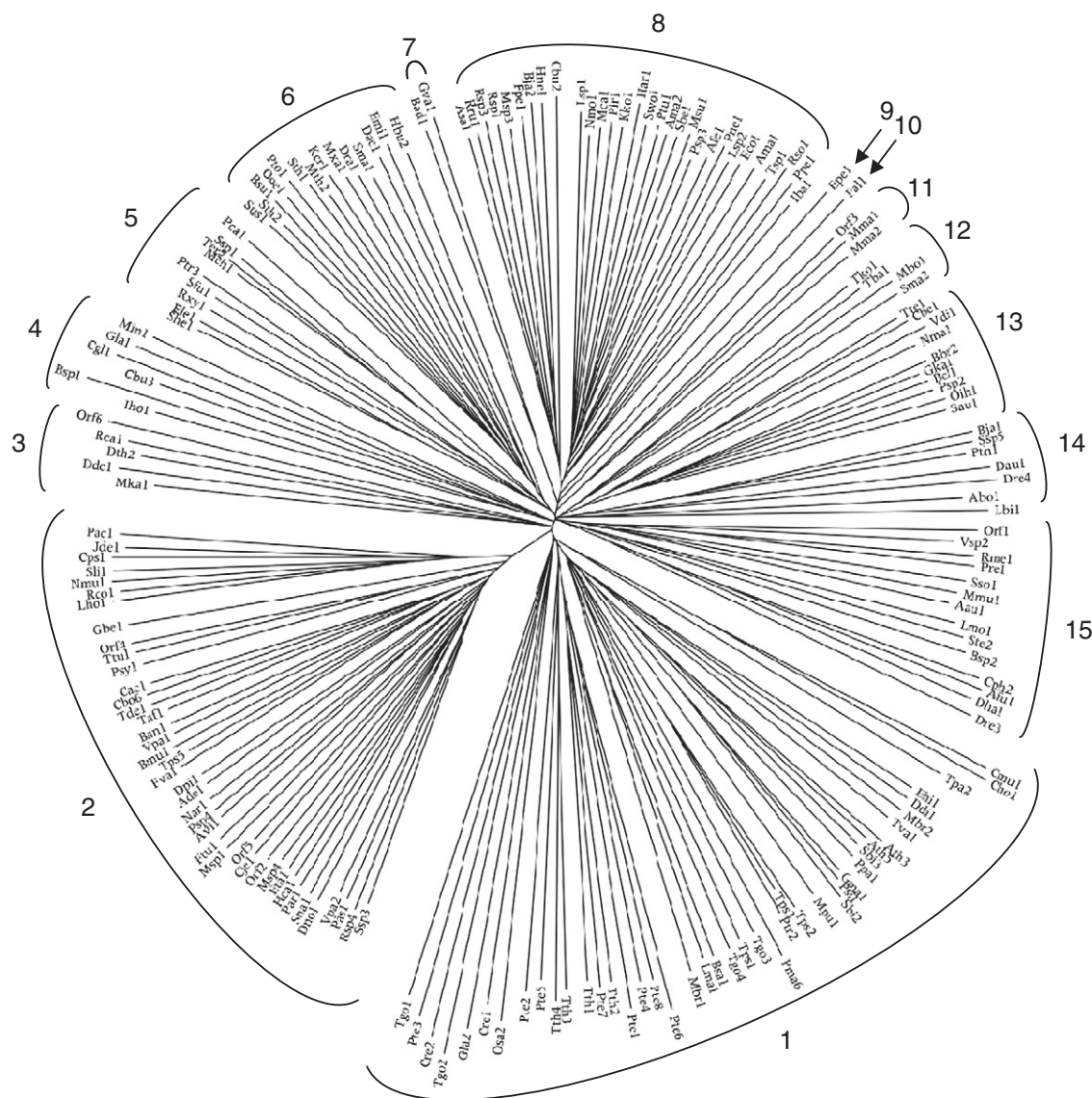
Fig. 1. Phylogenetic tree of the 189 TSUP family proteins included in this study. The tree was generated using the ClustalX multiple alignment and FigTree programs. Protein abbreviations and their descriptions are listed in Table 1 in a clockwise fashion starting from cluster 1. The positions of individual proteins within the phylogenetic tree are revealed in Fig. S1.
