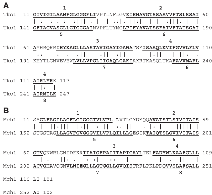
Fig. 4. Demonstration that 8 TMS TSUP family members arose by intragenic duplication of a primordial 4 TMS encoding genetic element. (A) GAP alignment of TMSs 1–4 of TSUP Tko1 ( Thermococcus kodakarensis ; gi# 57640914) with TMSs 5–8 of the same protein. Initial identification of repeat units was done using the IC program. The GAP program was run with default settings and 500 random shuffles. Residue identities are signified by vertical lines, while close and more distant similarities are signified by colons or periods, respectively. The numbers at both ends of each line signify the positions of the residues in the proteins. TMS positions were predicted using the TMHMM 2.0 program for this and subsequent comparisons. A comparison score of 26 S.D. was obtained. (B) GAP alignment of TMSs 1–4 of TSUP Mch1 ( Microcoleus chthonoplastes ; gi# 224407624) with TMSs 5–8 of Mch1. A comparison score of 17 S.D. was obtained.
