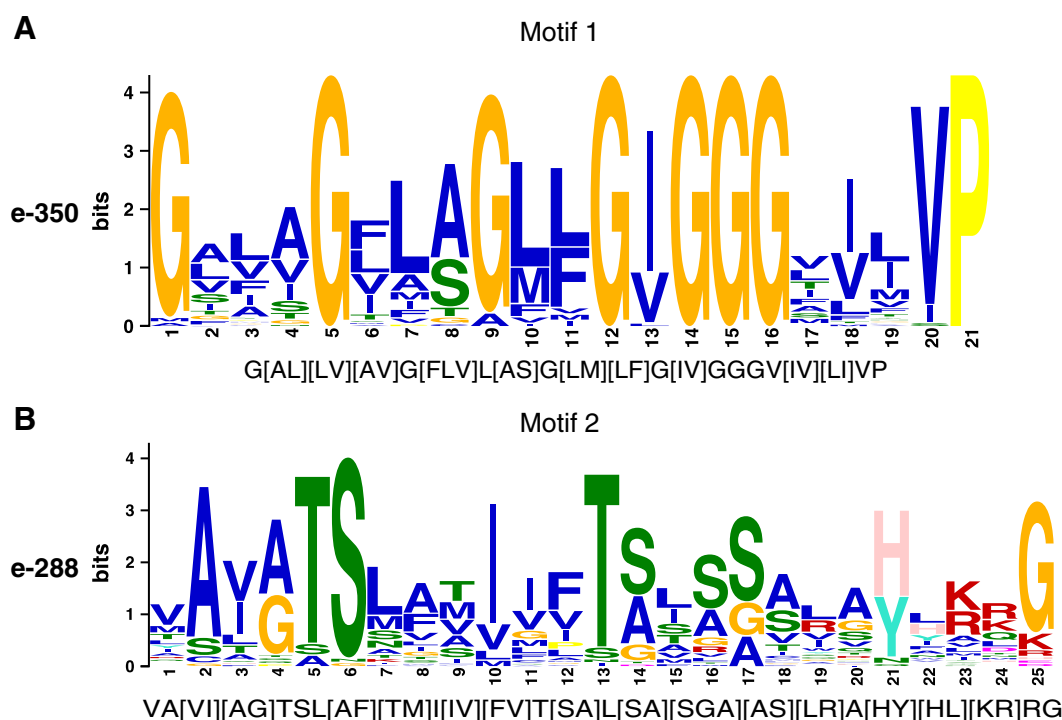
Fig. 5. (A and B) The two best conserved motifs found within the TSUP family as predicted by MEME. Corresponding statistical scores are presented on the y-axis. MAST predictions of motifs based on the MEME results are presented on the x-axis below each motif graphic.
