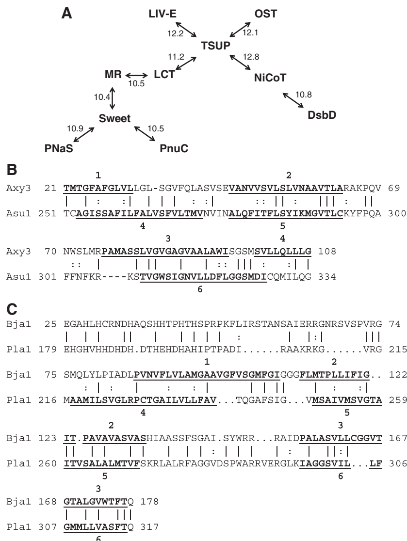
Fig. 6. (A) Rhodopsin superfamily homology established through the use of GSAT/GAP and the Superfamily Principle. Established Rhodopsin superfamily proteins from TCDB and their homologues were used to establish homology between all members of the ten families. GSAT/GAP scores, adjacent to the arrows, are expressed in terms of standard deviations (S.D.). (B) Homology between members of the TSUP and LCT families. GAP alignment of TMSs 1–3 of TSUP Axy3 ( Achromobacter xylosoxidans ; gi 311107599) with TMSs 4–6 of LCT Asu1 ( Ascaris suum ; gi 324511247). A comparison score of 11.2 S.D. was obtained with 43.8% similarity and 28.1% identity. (C) Homology between members of the TSUP and NiCoT families. GAP alignment of TMSs 1–3 of TSUP Bja1 ( Bradyrhizobium japonicum ; gi 27376265) with TMSs 4–6 of NiCoT Pla1 ( Parvibaculum lavamentivorans ; gi 154252649). A comparison score of 12.8 S.D. was obtained with 44.7% similarity and 36.4% identity.
